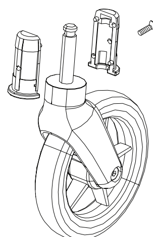
Front wheel with fork and plastic bushing.
