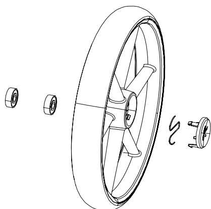
Rear wheel with bearings
