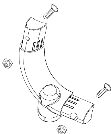
Front wheel connector
